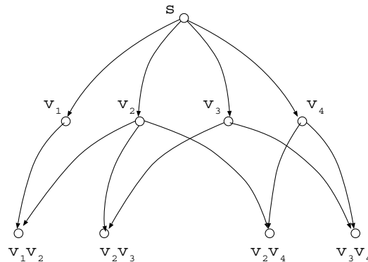
Fig. 3 Reduction from VERTEX COVER
